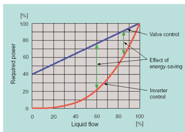
Liquid flow and power characteristics
